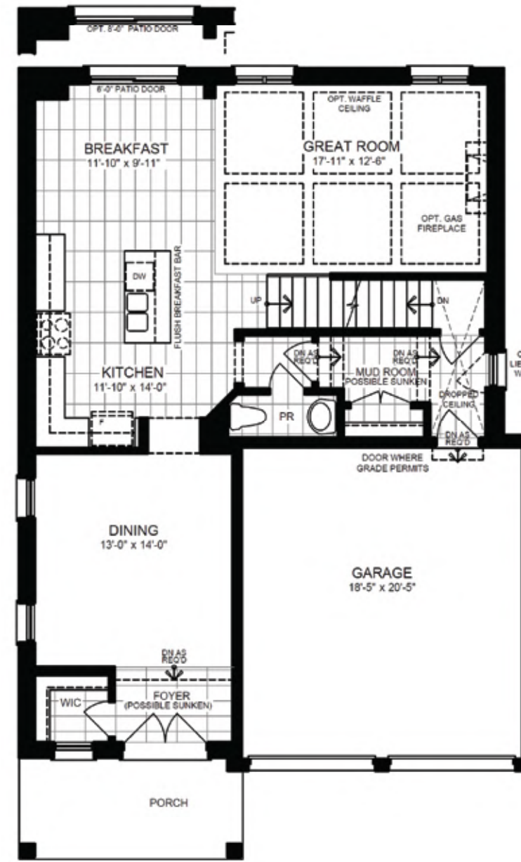
MAIN FLOOR PLAN ELEVATION 'A'
