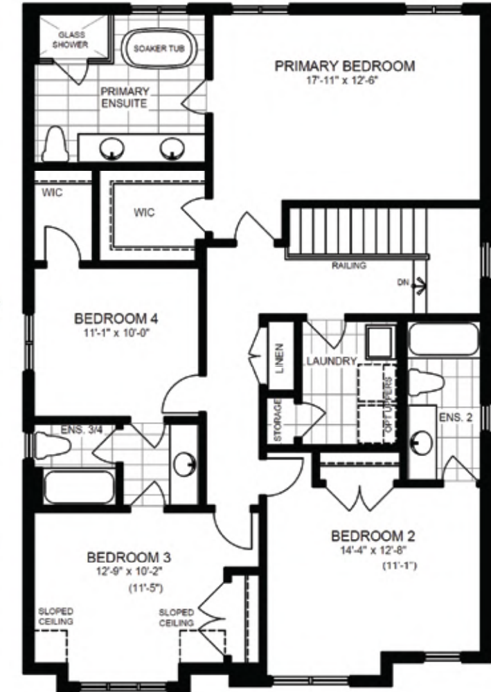
SECOND FLOOR PLAN ELEVATION 'A'
