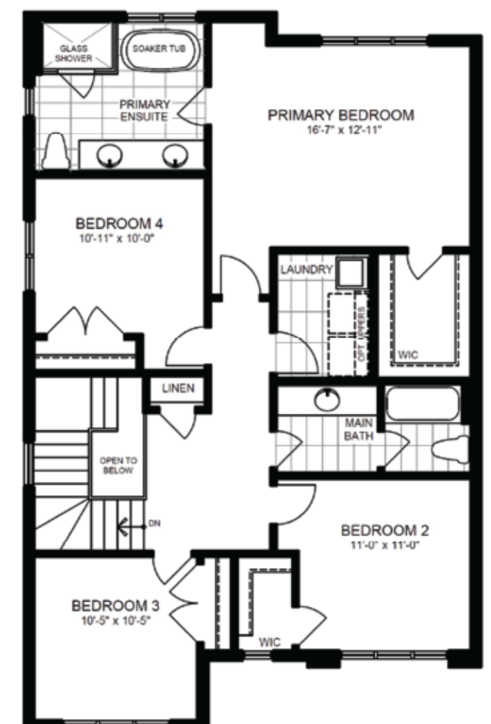
SECOND FLOOR PLAN ELEVATION 'A'
