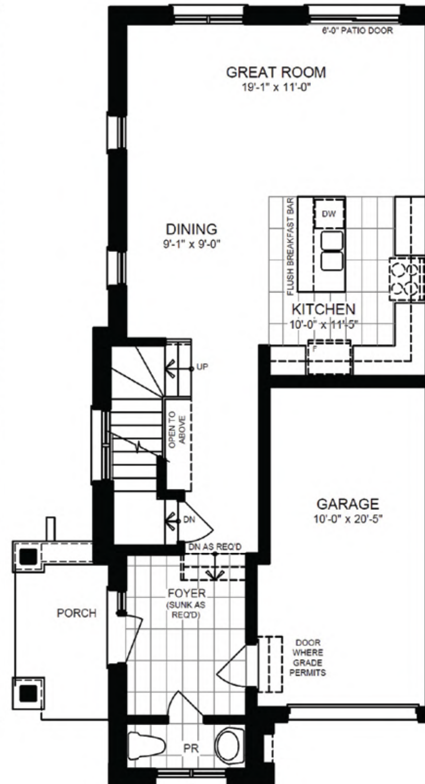
MAIN FLOOR PLAN ELEVATION 'A4' CORNER
