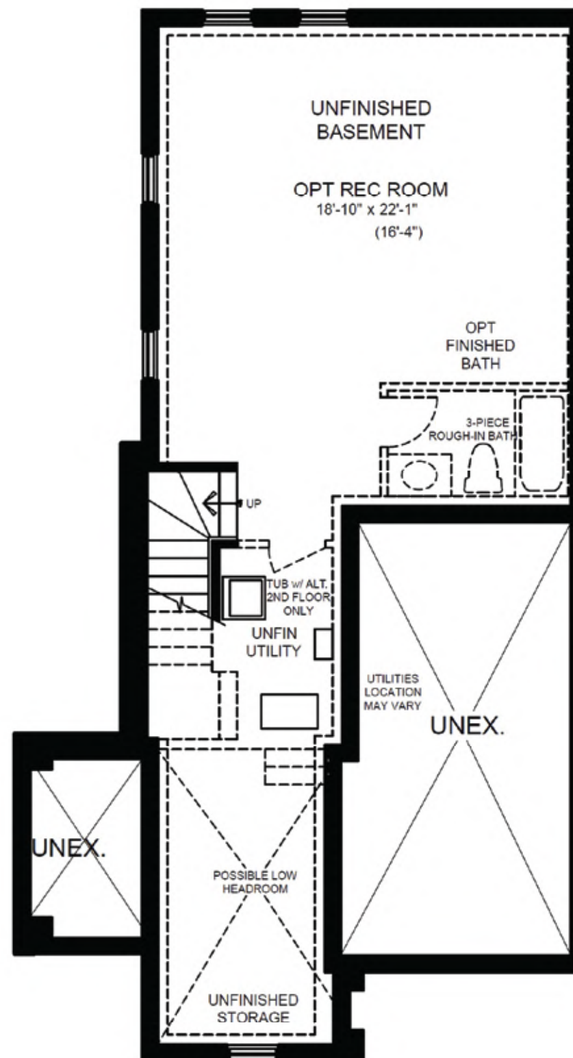
BASEMENT PLAN ELEVATION 'A4' CORNER
