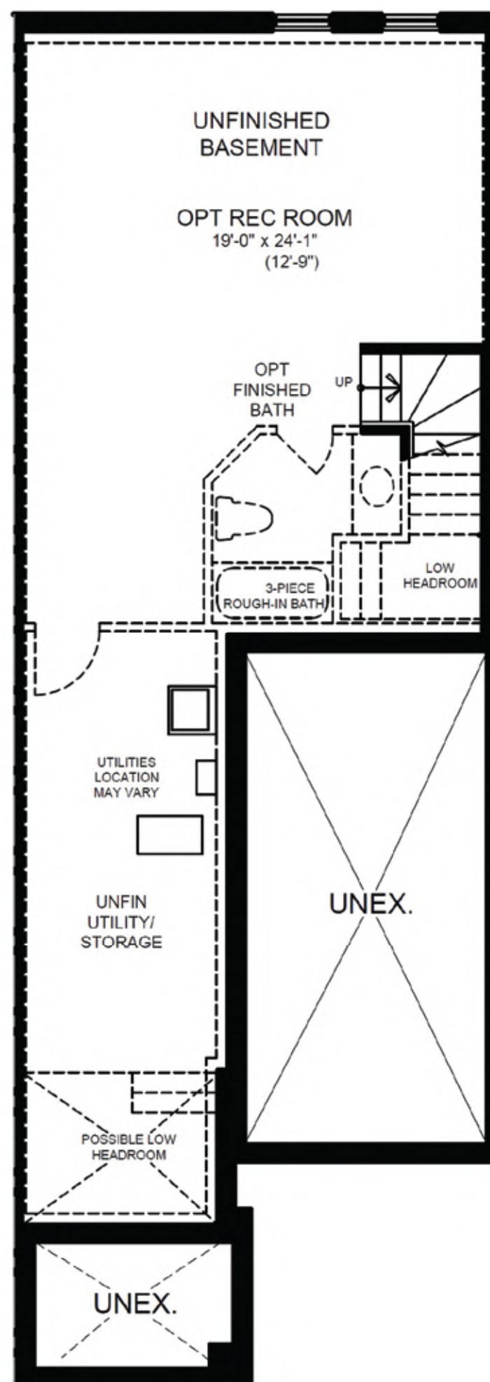
BASEMENT PLAN ELEVATION 'A1' & 'A2'
