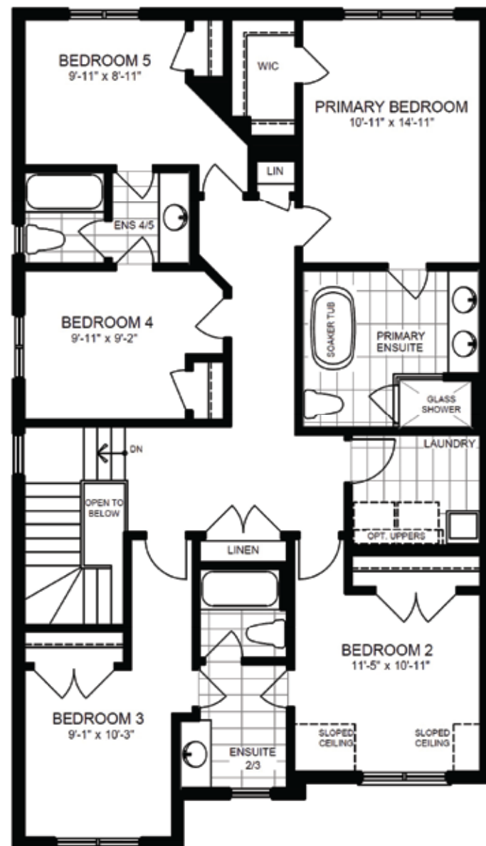
5 BEDROOM SECOND FLOOR PLAN ELEVATION 'A'
