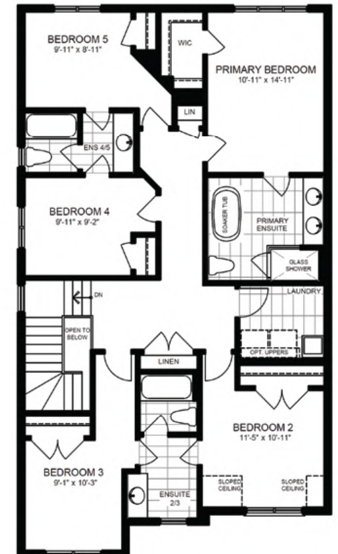
5 BEDROOM SECOND FLOOR PLAN ELEVATION 'A'
