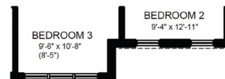
PARTIAL SECOND FLOOR PLAN ELEVATION 'A2'
