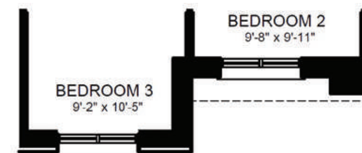
PARTIAL SECOND FLOOR PLAN ELEVATION 'B2'
