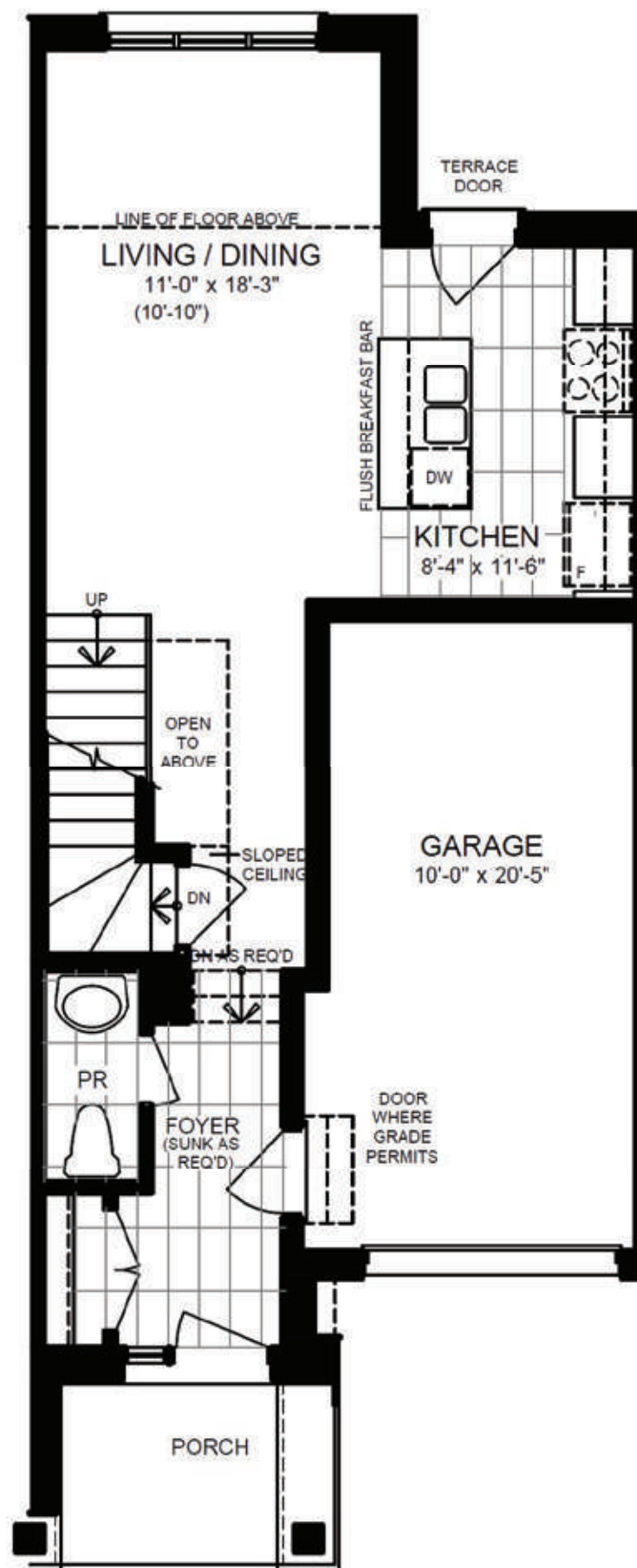
MAIN FLOOR PLAN ELEVATION 'A1' & 'A2'
