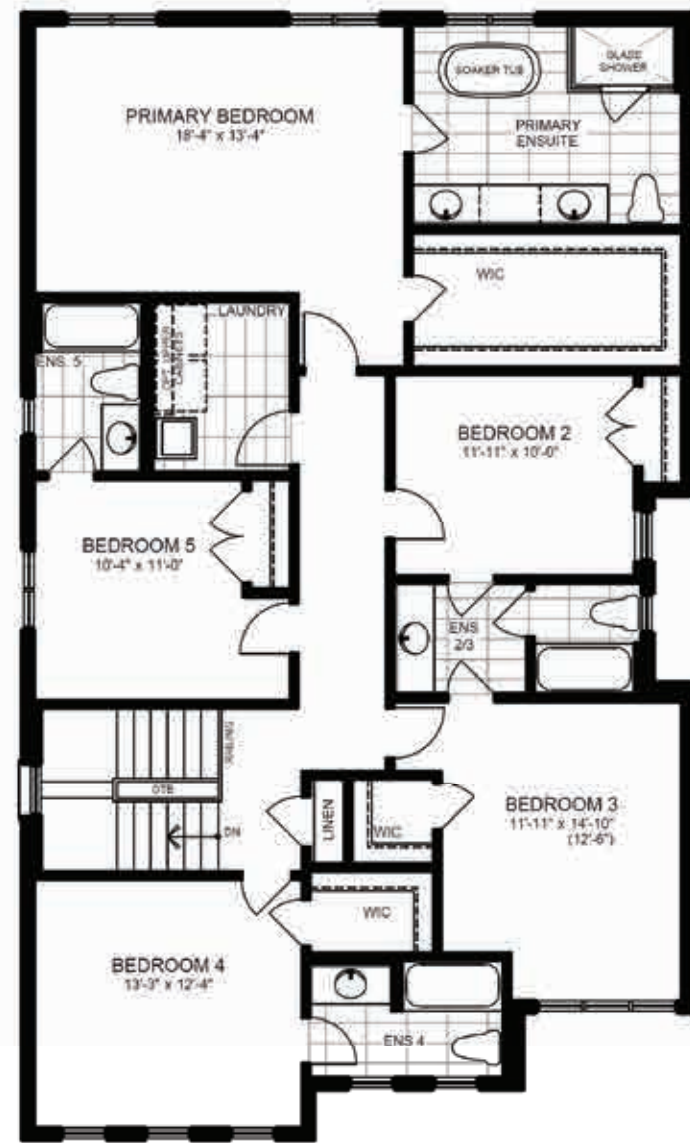
5 BEDROOM SECOND FLOOR PLAN ELEVATION 'A'
