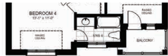
5 BEDROOM PARTIAL SECOND FLOOR PLAN ELEVATION 'B'
