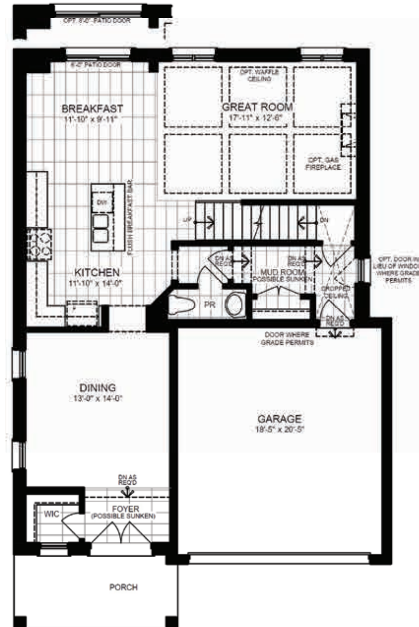
MAIN FLOOR PLAN ELEVATION 'A'
