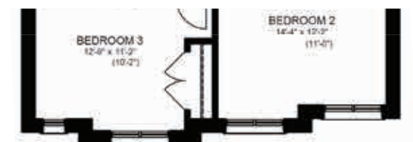
PARTIAL SECOND FLOOR PLAN ELEVATION 'C'
