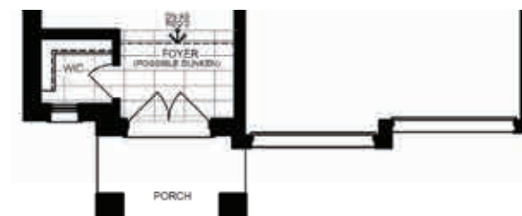
PARTIAL MAIN FLOOR PLAN ELEVATION 'C'
