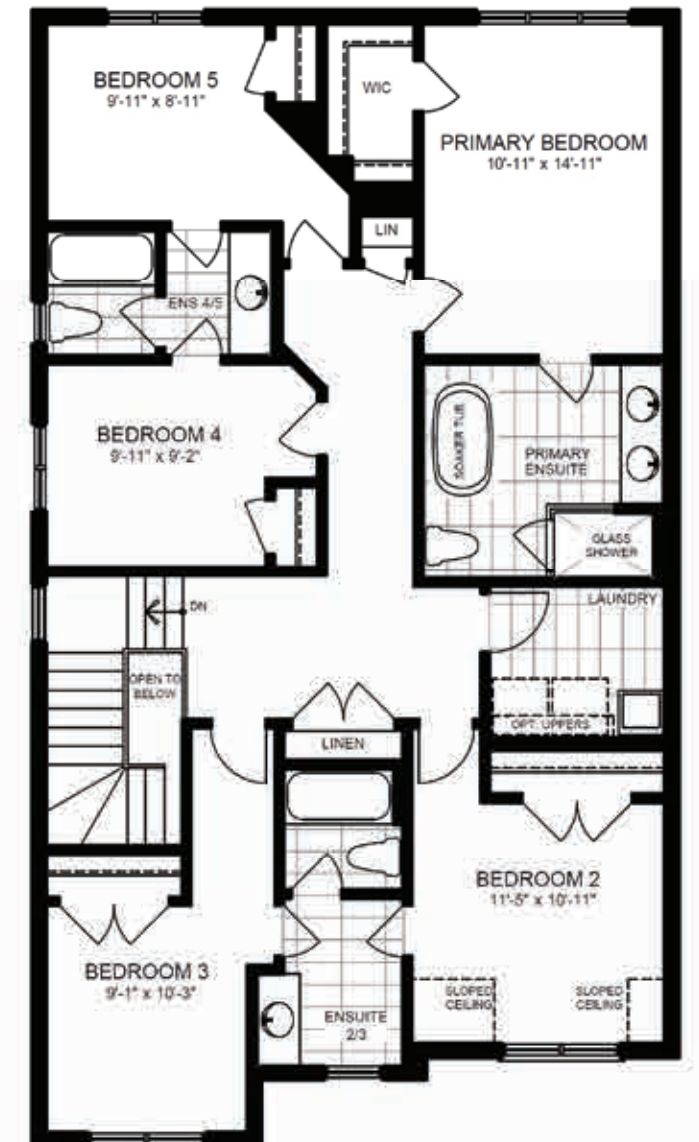
5 BEDROOM SECOND FLOOR PLAN ELEVATION 'A'
