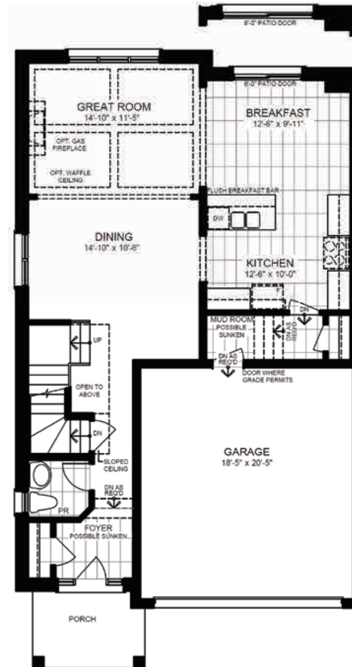
MAIN FLOOR PLAN ELEVATION 'A'
