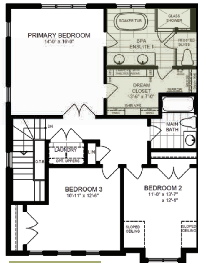
THE SORBARA SERIES SECOND FLOOR PLAN W/ SPA ENSUITE & DREAM CLOSET ELEVATION 'A'
