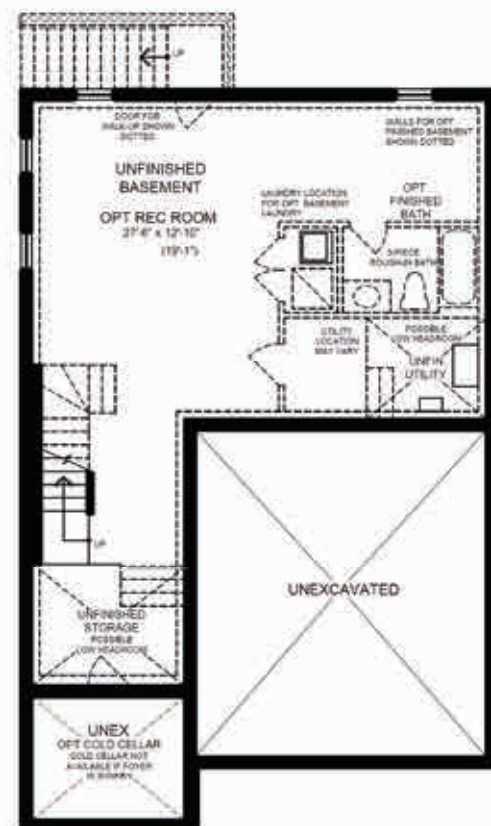
BASEMENT FLOOR PLAN ELEVATION 'A'
