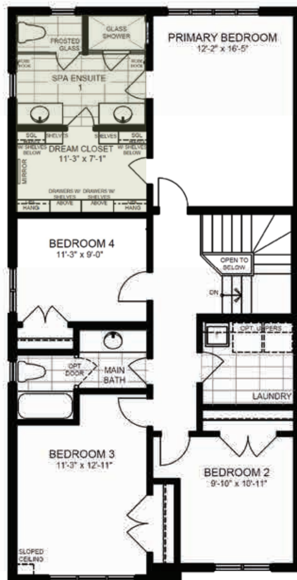
THE SORBARA SERIES SECOND FLOOR PLAN W/ SPA ENSUITE & DREAM CLOSET ELEVATION 'A'
