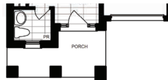
PARTIAL MAIN FLOOR PLAN ELEVATION 'C'
