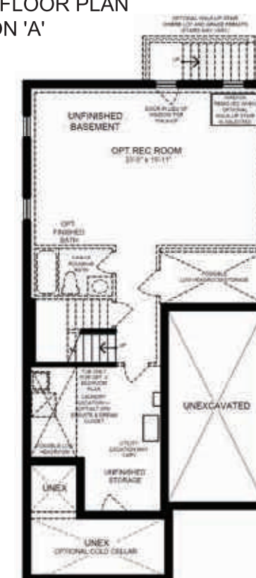
BASEMENT PLAN ELEVATION 'A'
