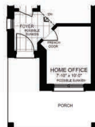
PARTIAL MAIN FLOOR PLAN ELEVATION 'A' OPT. HOME OFFICE
