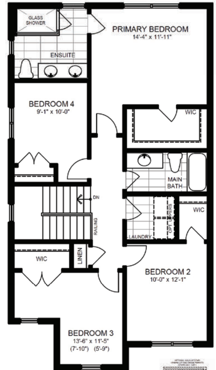
4 BEDROOM SECOND FLOOR PLAN ELEVATION 'A'
