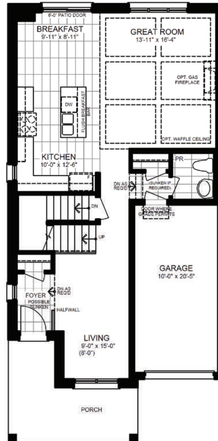
MAIN FLOOR PLAN ELEVATION 'A'
