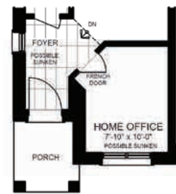
PARTIAL MAIN FLOOR PLAN ELEVATION 'B' OPT. HOME OFFICE
