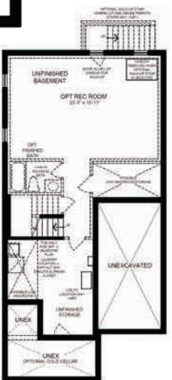
BASEMENT PLAN ELEVATION 'A'
