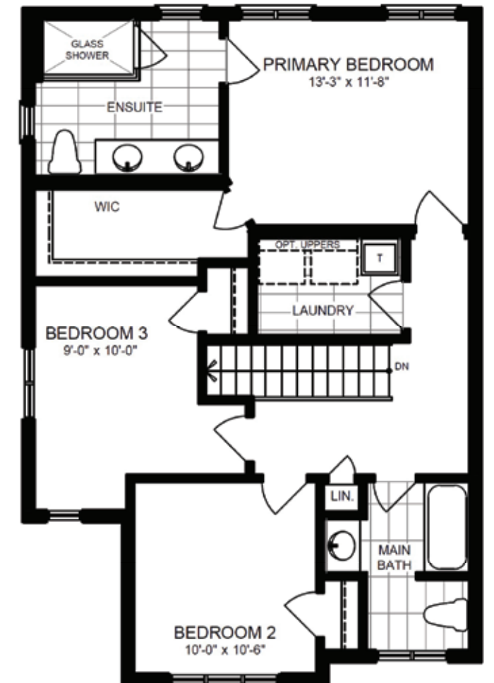
SECOND FLOOR PLAN ELEVATION 'A'
