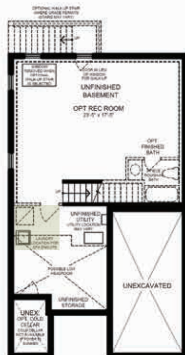
THE SORBARA SERIES BASEMENT PLAN ELEVATION 'A'
