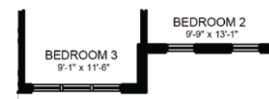
PARTIAL SECOND FLOOR PLAN ELEVATION 'A2'
