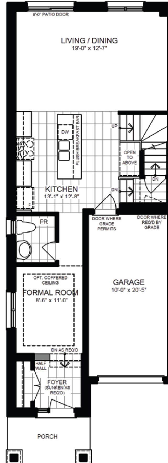
MAIN FLOOR PLAN ELEVATION 'A3' END
