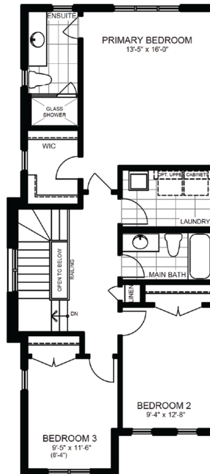
SECOND FLOOR PLAN ELEVATION 'A4' CORNER
