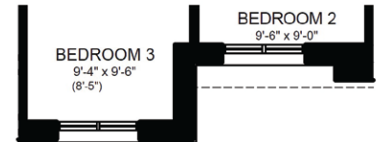
PARTIAL SECOND FLOOR PLAN ELEVATION 'B2'
