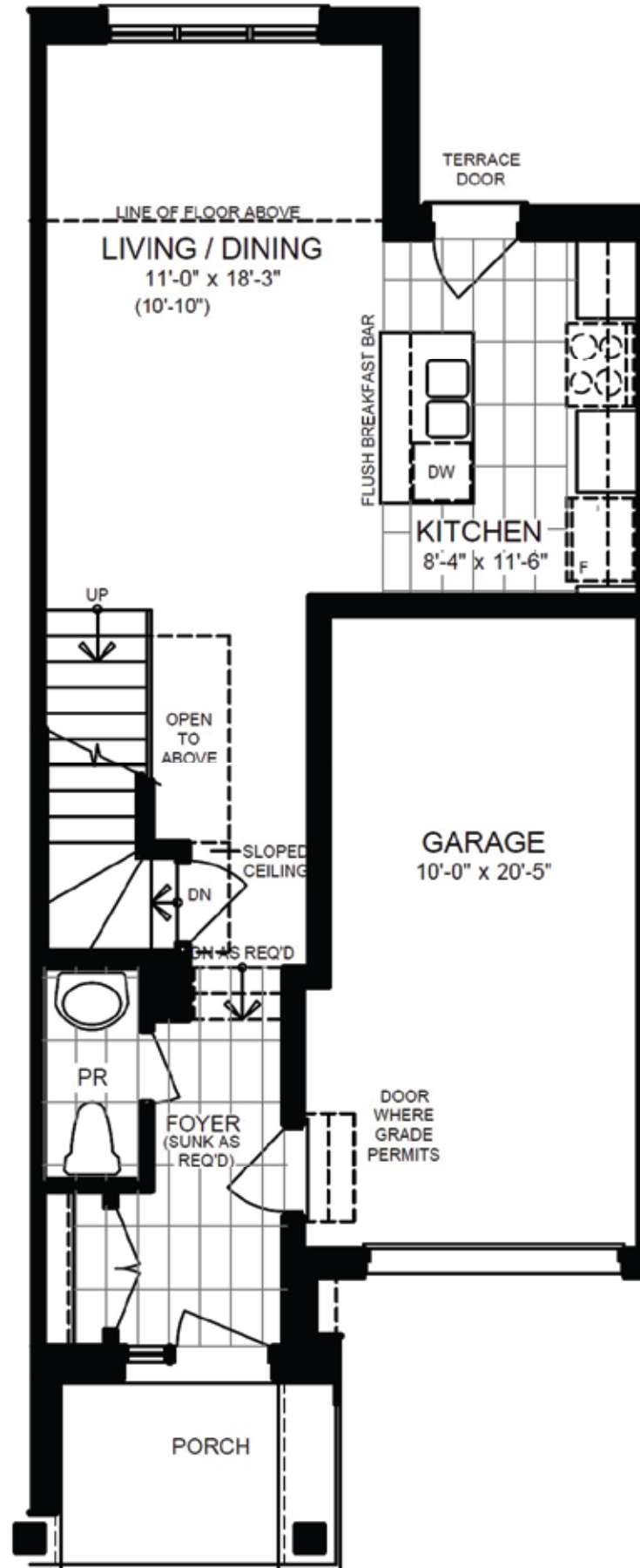
MAIN FLOOR PLAN ELEVATION 'A1' & 'A2'
