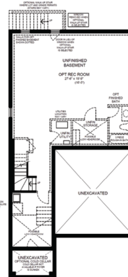
BASEMENT PLAN ELEVATION 'A'
