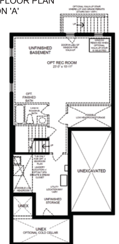
BASEMENT PLAN ELEVATION 'A'
