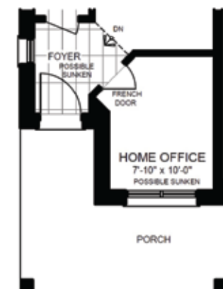
PARTIAL MAIN FLOOR PLAN ELEVATION 'A' OPT. HOME OFFICE
