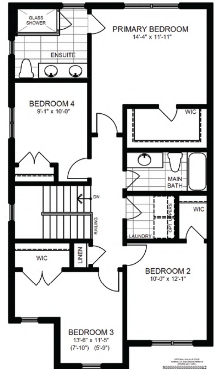
4 BEDROOM SECOND FLOOR PLAN ELEVATION 'A'
