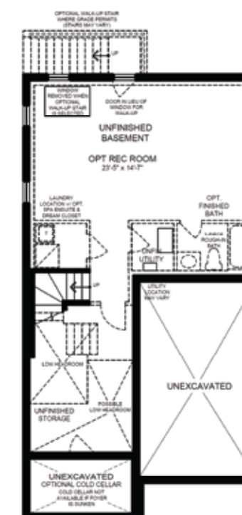
BASEMENT PLAN ELEVATION 'A'
