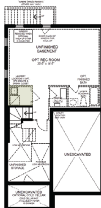
THE SORBARA SERIES BASEMENT PLAN ELEVATION 'A'
