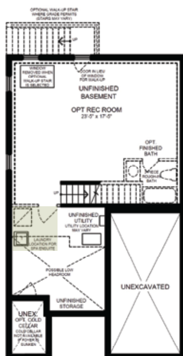
THE SORBARA SERIES BASEMENT PLAN ELEVATION 'A'
