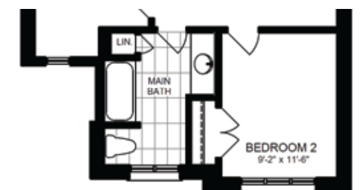
PARTIAL SECOND FLOOR PLAN ELEVATION 'B'
